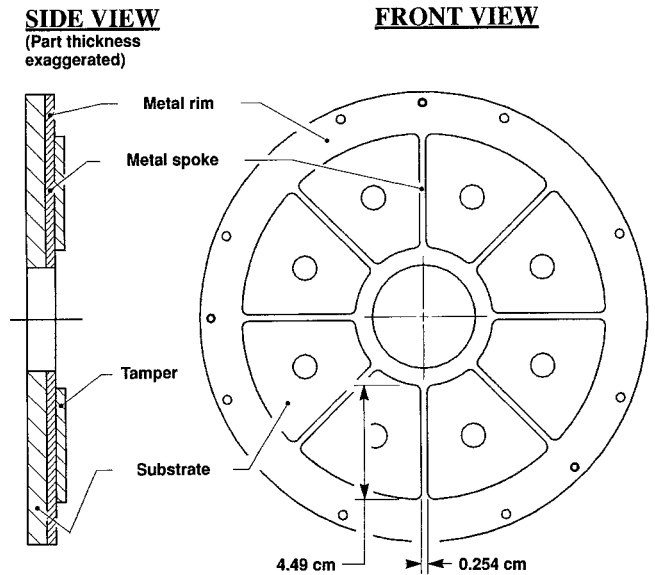
Figure 3. Front and side views of a typical 8-spoke fuse.
