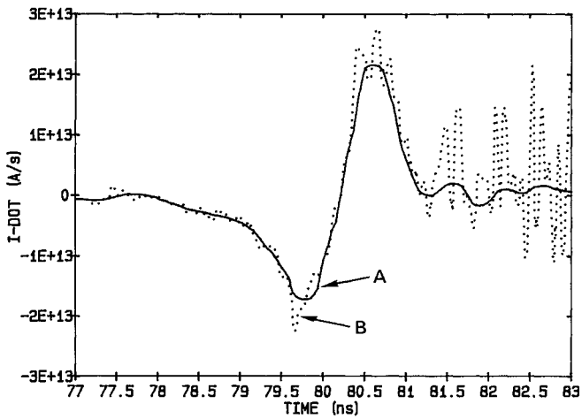
Figure 5. Output I-dot measured behind the 16-spoke fuse. A) B-dot probe measurement (TEK 7104) B) B-dot probe measurement (TEK 7250)
