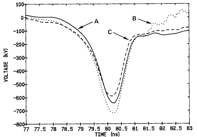
Figure 6. Output voltage measured behind the 16-spoke fuse. A) B-dot probe measurement (TEK 7104) B) B-dot probe measurement (TEK 7250) C) CVR measurement (TEK 7104)
