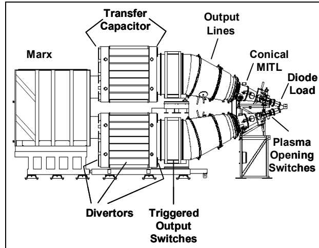
Figure 1. DECADE Quad in the Large Area Bremsstrahlung configuration.
