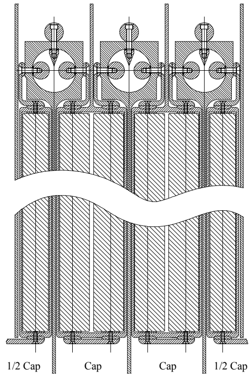
Figure 8. Conceptual cross-section of Marx stages using switch-with-barrier-approach.
