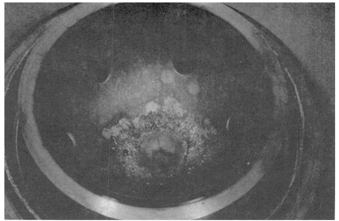
Figure 2. Photograph of lower cathode delimiter showing electrode damage.
