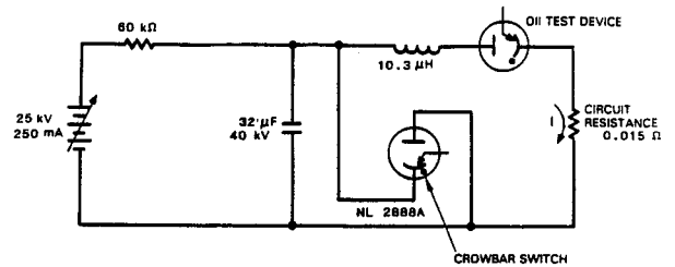
Figure 5. Major components of OII test circuits for initial testing at 10 to 15 kA peak current.
