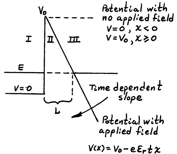
Fig 1. Potential barrier outside an electrode due to an applied electric field
