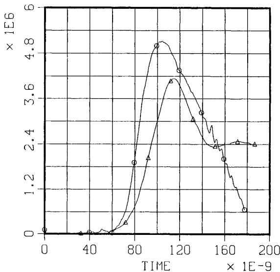
Figure 6. The current measured at the stack (circles) compared with the current near the load (triangles).
