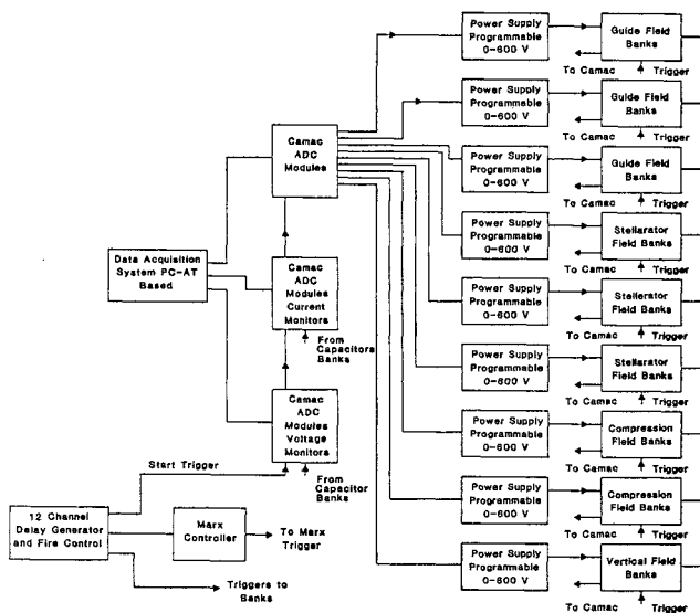
Figure 4. Camac crate based control and diagnostic system.
