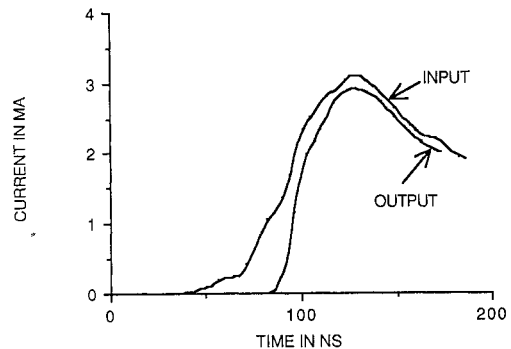
Figure 17 - POS Performance
