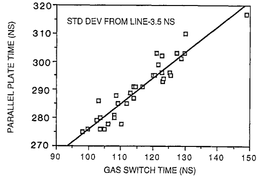
Figure 10 - Water Switch Jitter
