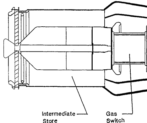
Figure 5 - Water Capacitor
