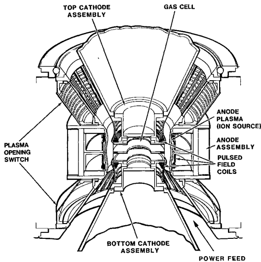
Figure 16 - POS-Diode Drawing
