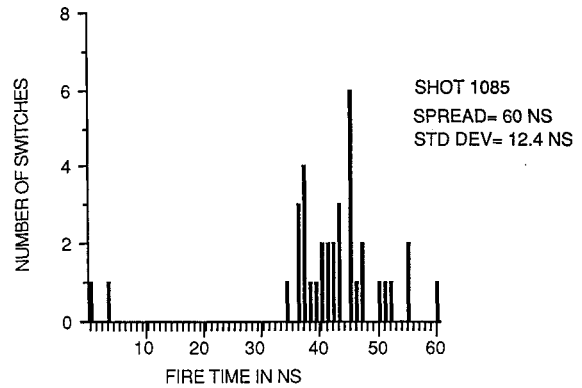
Figure 7 - PBFA II Typical LTS Performance
