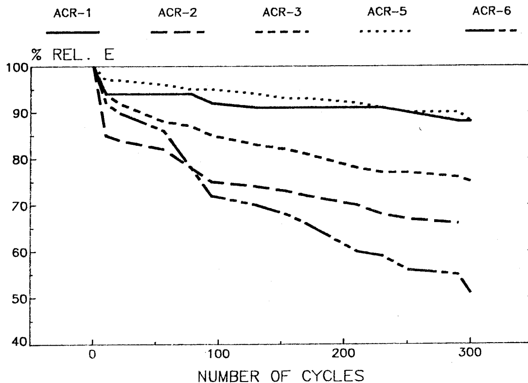
Figure 9. Relative dynamic modules of elasticity for five test specimens
