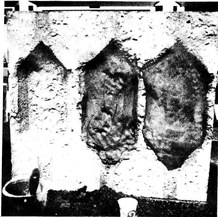
Figure 4. Application to vertical surfaces
