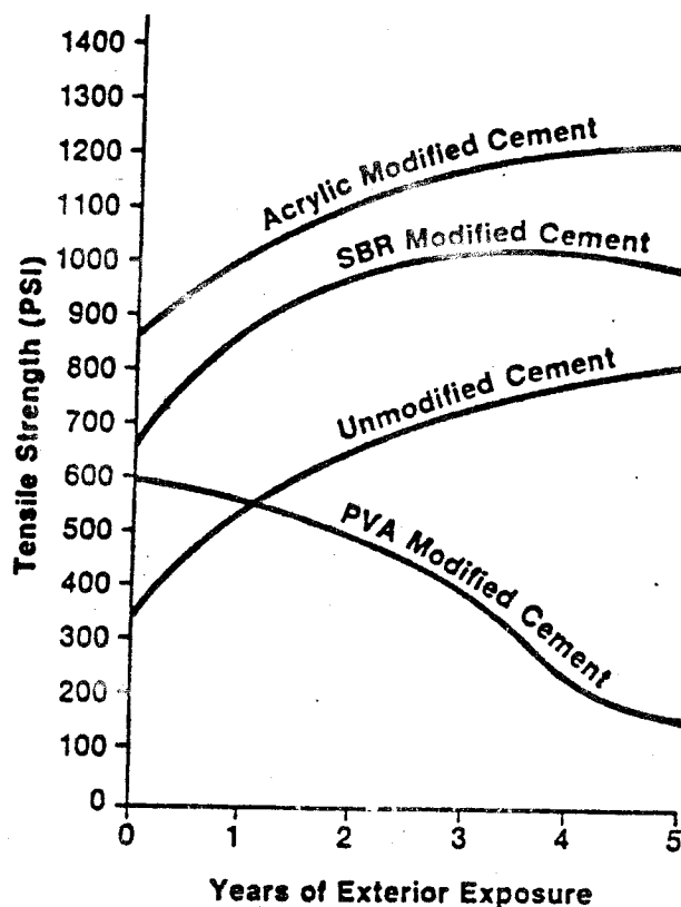
Figure 2. Comparative durability of polymer-modified cements (Rohm and Haas Company 1982)
