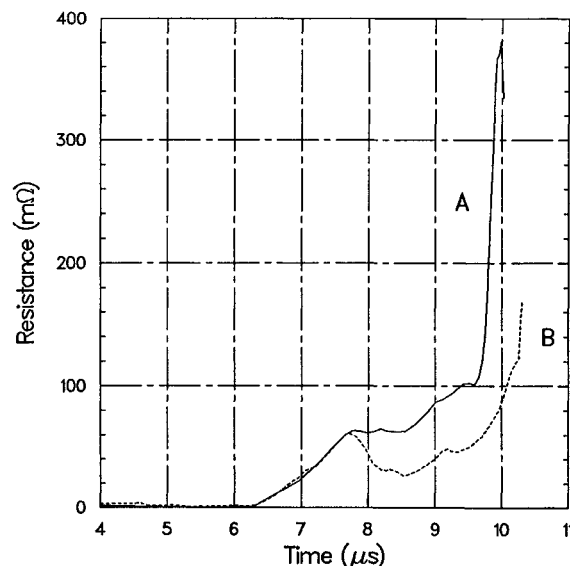
Figure 2. Resistance curves produced by two different die patterns operating at different energy dissipation limits. ~125 kJ were dissipated in test A while 450 kJ were dissipated in test B.
