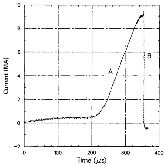
Figure 4. Large scale EFF test results. Curve A is the current pulse conducted (and interrupted) by the EFF. Curve B is the current transferred to a 10 nH load. On this scale, curve B, the load current, nearly disappears behind the decaying curve A.
