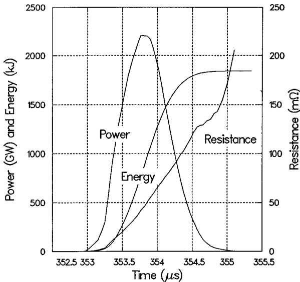
Figure 6. Resistance generated by the large scale EFF, the resulting power pulse and total I^2R energy dissipated. The time scale is the same as Fig. 4. The die pattern in this test is the same as that of curve B in Fig. 2, and the resistance profile compares favorably with 1.5 times the curves in Fig. 2.
