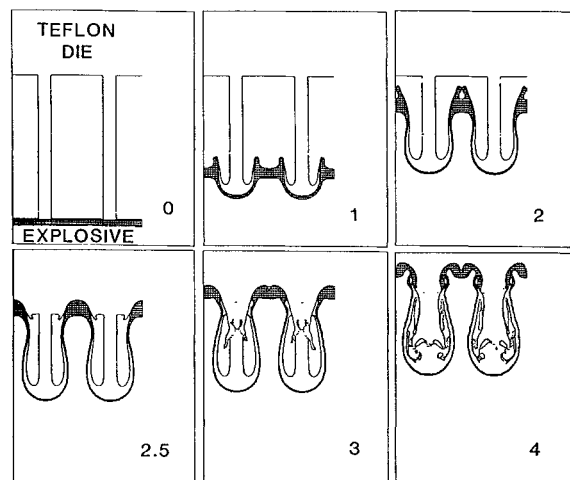
Figure 1. Two-dimensional hydrodynamics code simulation of the evolution of an explosively formed fuse. The simulation shows explosives driving an aluminum conductor (cross hatched) into a tefflon die. The numbers in each frame are the time in microseconds from the initial motion of the aluminum. Fuse action begins to occur at ~2 \mu s.
