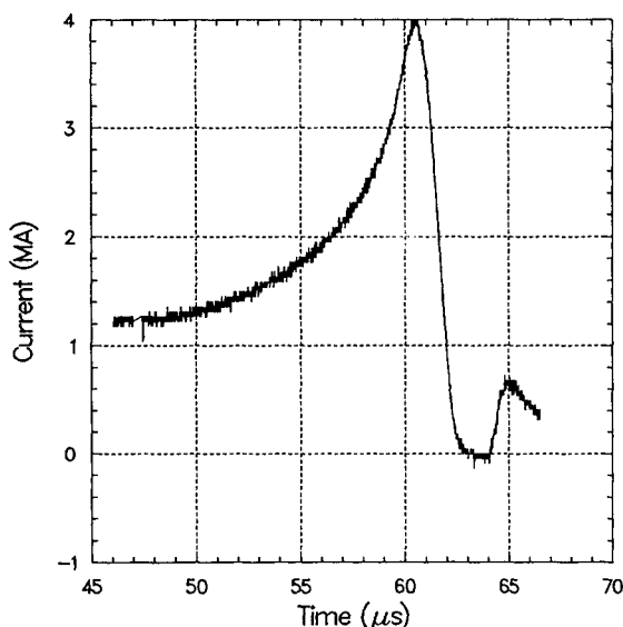
Figure 3. EFF current profile from fuse load test. The reconnection at 64- to 65- \mu s is due to a voltage >150 kV applied by the bursting fuse, and is consistent with an EFF resistance >200 m \Omega . The current pulse begins at ~15 \mu s on this time scale.
