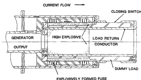
Figure 9. Side view of an advanced EFF design shown attached to a coaxial generator output and a coaxial dummy load. Arrows show initial conduction path. Surface discharge closing switch diverts current to load return conductor when EFF opens. Both a simultaneously initiated inner cylinder and an outer shell of explosives are required.
