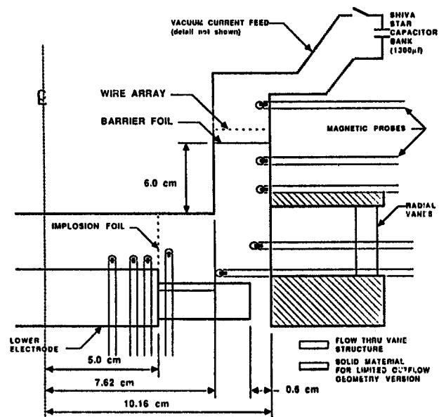
Figure 1. Plasma flow switch geometry.
