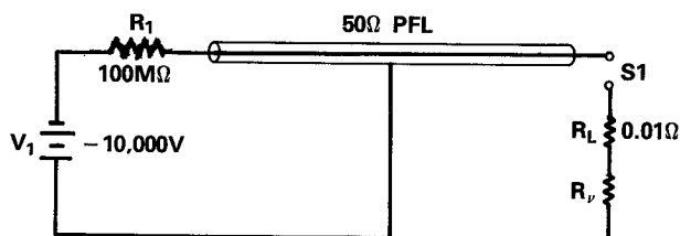
FIGURE 8. PFL WITH LOSSY SPARK GAP MODEL
