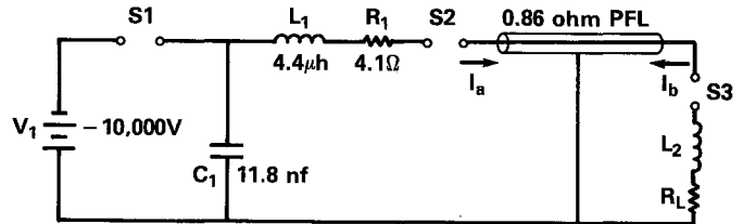
FIGURE 1. BASIC CIRCUIT DIAGRAM
