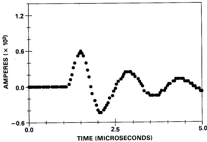
b. OUTPUT CURRENT I_b FROM PFL
