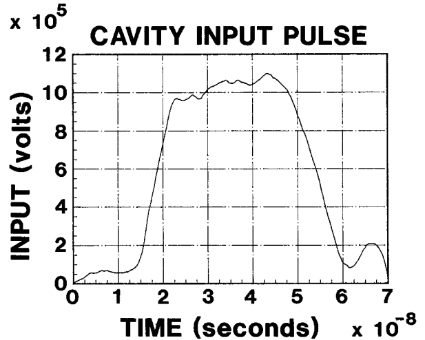
Fig. 5. PFL output pulse used as cavity input to the circuit model calculations
