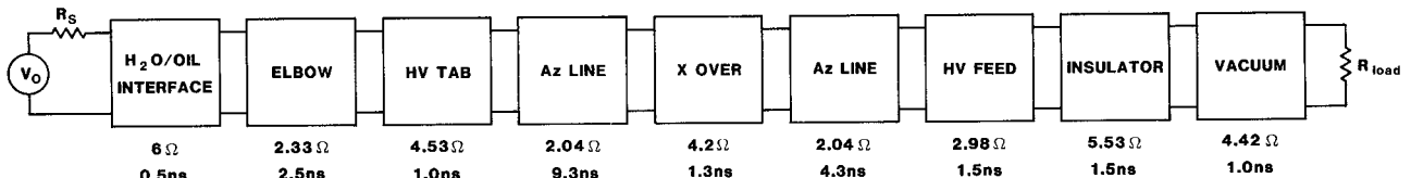
Fig. 4. SCREAMER circuit model of the cavity
