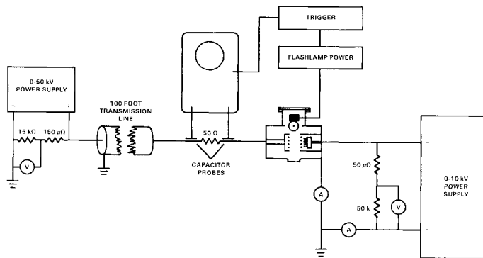
Fig. 4. Test set-up
