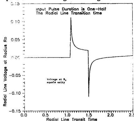
Figure 8. Computer RTL Voltage Transformations
