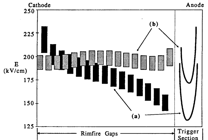
Figure 1. JASON-Derived Plots of the PBFA-II Gas Switch E-Field Distribution. Curve (a): Original Configuration. Curve (b): Final Modified Configuration.
