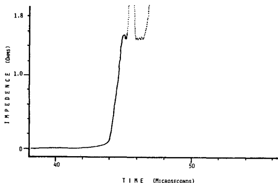
Figure 9 Fuse Impedance
