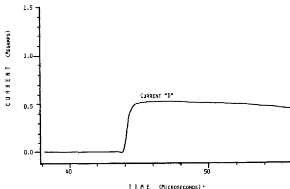
Figure 10 Load Current
