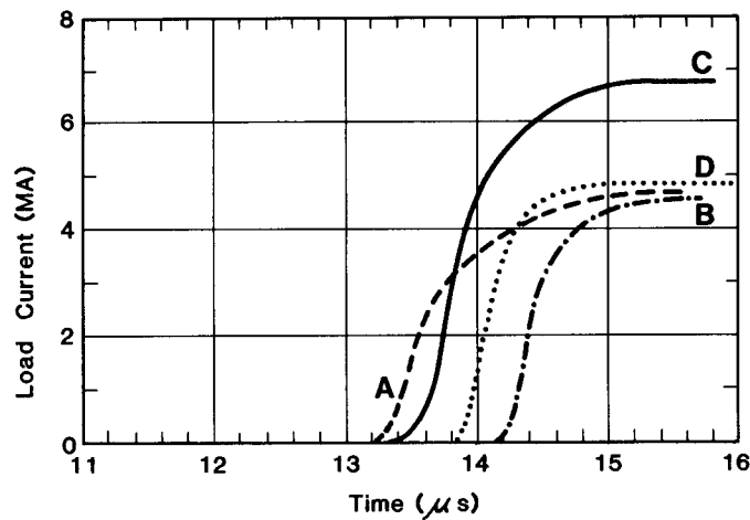
Fig. 6. Load pulses for tests shown in Fig. 5.
