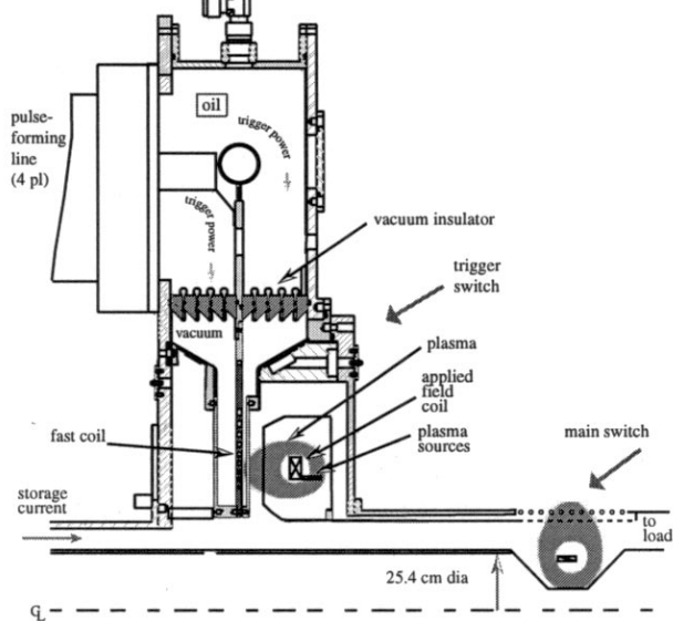
Figure 3. Cross-sectional view of the amplified-trigger POS.
