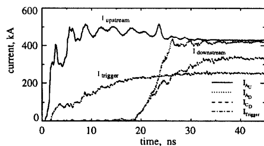
Figure 5. Simulation currents.
