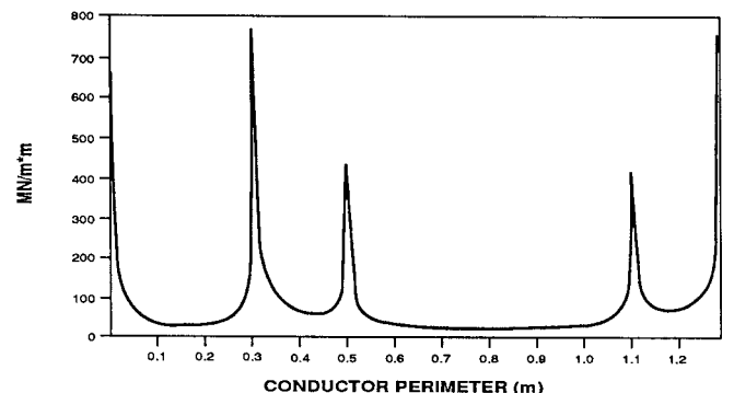
Figure 4c. Magnetic loading on surface
