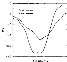
Fig. 2. Output Voltage Waveforms from the Previous and Present RADLAC II.
