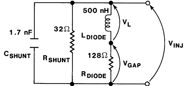
Fig. 5. LRC Load Circuit Model.
