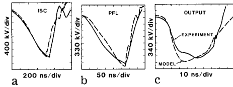
Fig. 4. Comparison of Simulated and Measured Waveforms.
