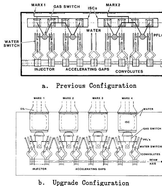
Fig. 1. Top View of Water Tank Hardware Layout.
