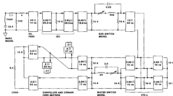
Fig. 3. Circuit Schematic Representing a 1/4 Module of RADLAC II.
