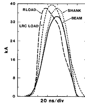
Fig. 6. Comparison of Simulated, Shank, and Beam Currents.
