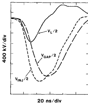
Fig. 7 Total Injector, A-K Gap, and LdI/dt Voltage Waveforms.
