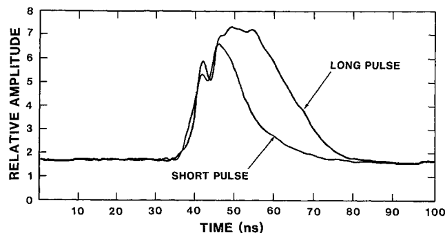
Fig. 9 Comparison of full and shortened laser pulses
