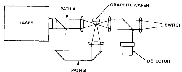
Fig. 8 Experimental arrangement used to shorten laser pulses
