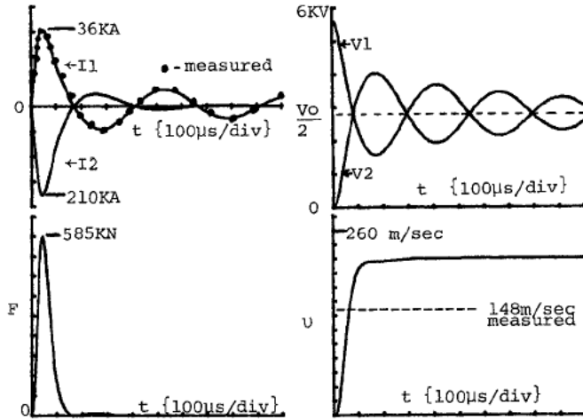
Figure 6: Computer generated curves compare to measurements for the following case: L_1 = 14\mu H , C_1 = C_2 = 828\mu F , R_1 = 34m\Omega , L_S = 1\mu H , Z_L = .035m , L_2 = .32\mu H , R_2 = .65m\Omega , m = .115 Kg, and K_0 = .89
