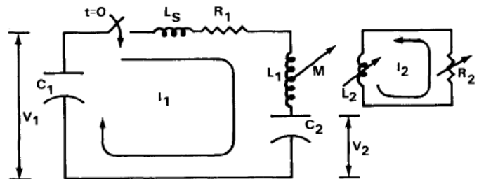
Figure 3: Circuit model of twin capacitor-bank device
