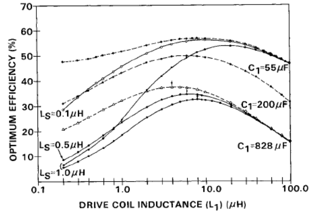
Figure 7: Computer generated optimum efficiency curves as a function of L_1 , C_{eff} , and L_S . R_1 = 15.6m\Omega , R_2 = 1.1m\Omega , L_2 = .32\mu H , K_0 = .89 , Z_L = .035m , and m = .1 Kg
