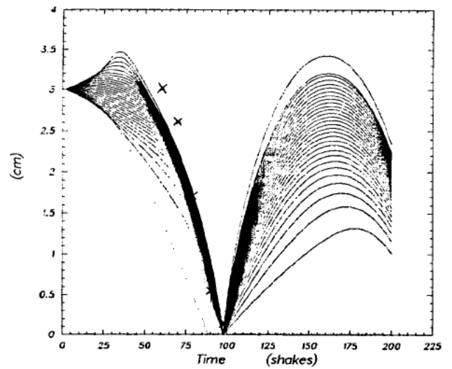
Calculated implosion of the plasma load using the 1-D MHD model and the measured current from the Pioneer I-2 experiment. The (x)'s indicate the effective radius of the load determined from its inductance.
