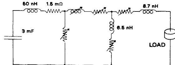
Equivalent circuit used for the Pioneer I preshot calculation.
