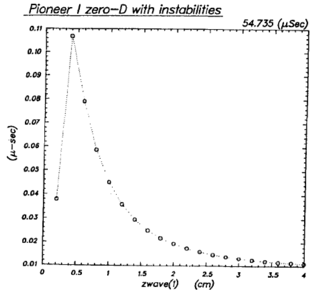
Thermalization time as a function of wave length of R-Z perturbation calculated with a heuristic model of magnetically driven Rayleigh-Taylor instabilities.
