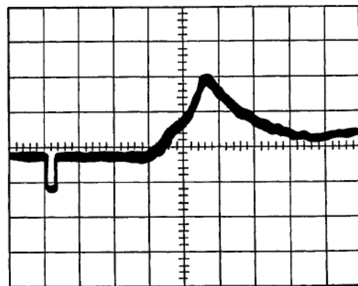
Fig. 5 Signal from the visible diode, for Pioneer I-2. Vertical axis: 5 V/div, horizontal axis: 500 ns/div. The negative fiducial began at a reference time of 76.32 \mu s.
