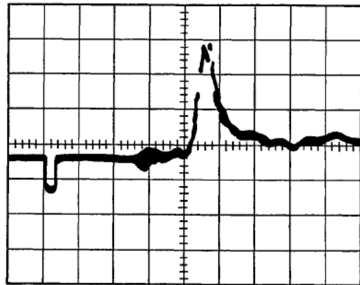
Fig. 4 Signal from XRD channel 4, for Pioneer I-2. Vertical axis: 5 V/div, horizontal axis: 500 ns/div. The negative fiducial began at a reference time of 76.32 \mu s.
