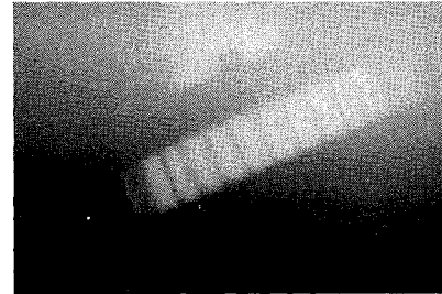
Fig.10b A record of the fifth (time integrated) channel of "4-eyes", obtained for Pioneer I-2. This channel records visible emission from the foil for all phases: initiation, run in and implosion. Dark lines are conductor vanes, spaced 8.7 mm apart.
