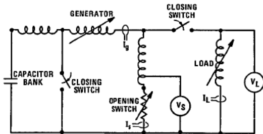
Fig. 1 Circuit diagram of the Pioneer I active inductive storage driver and load.
