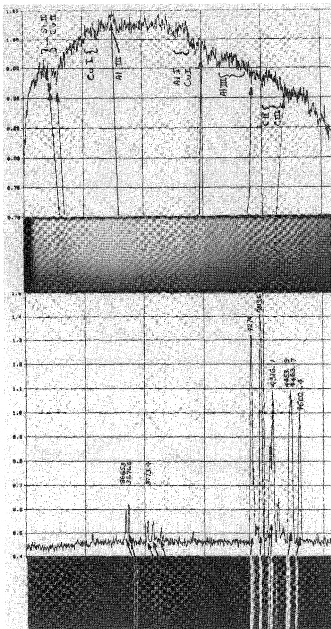
Fig. 6 The spectrum recorded by the visible spectrometer for Pioneer I-2. The upper portion shows the spectrum and the corresponding densitometer trace. The lower portion shows the krypton calibration spectrum and its densitometer trace. Vertical axis gives the specular density, horizontal axis gives the wavelength in Angstroms.
