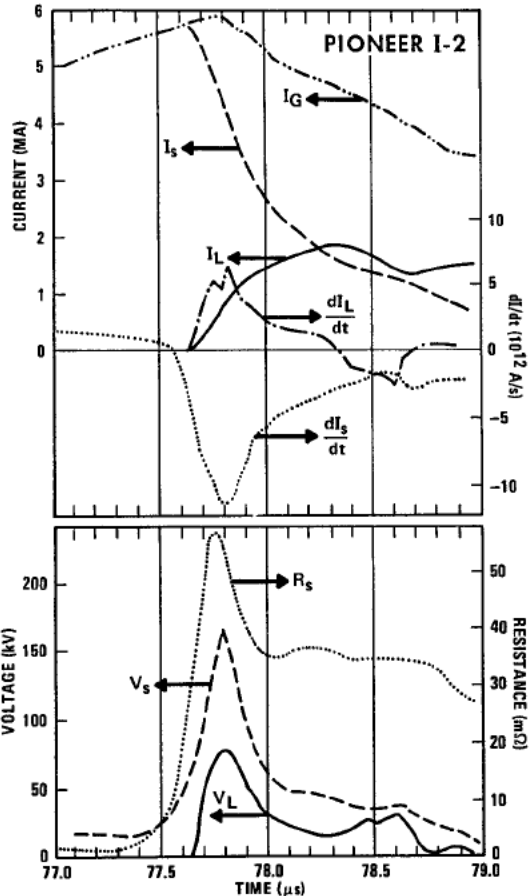
Fig. 2 Electrical characteristics for Pioneer I-2. Opening switch reaches maximum resistance at \sim 77.7 \mu\text{s} , pinch occurs at \sim 78.6 \mu\text{s} .
