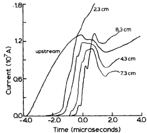
Figure 4. QF-5 gun magnetic probe data
