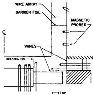
Figure 2. QF-5 Magnetic Probes
