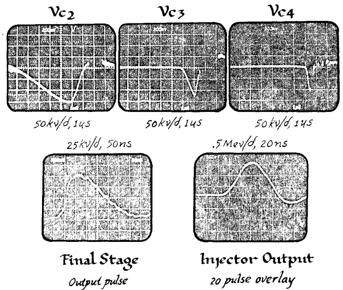
Fig 6 Waveforms
