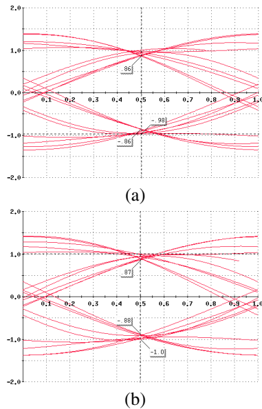
Figure 8 BPSK eye diagrams (BW = 2 GHz, 3.1 dB IBO) (a) SPW (b) MAFIA
