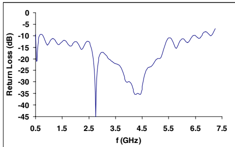
Figure 2 Return loss for simulated XWING coupler design
