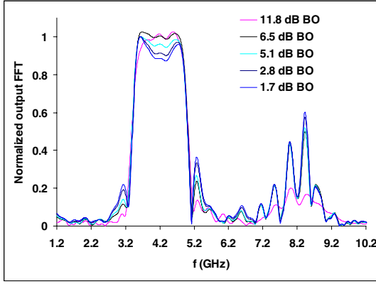
Figure 5 Simulated normalized output spectrum using wideband excitation (BW = 2 GHz)
