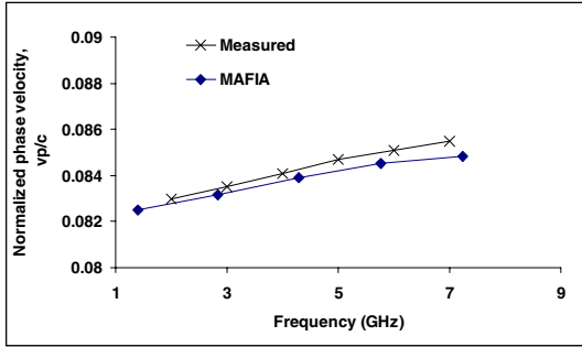
Figure 1 Measured and simulated normalized phase velocity
