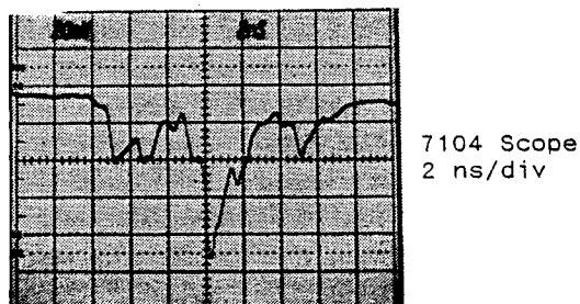
Figure 6. Q-switched laser pulse shape.
