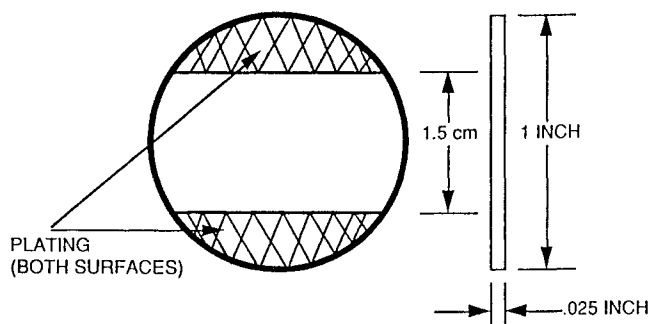
Figure 1. Solid switch wafer.
