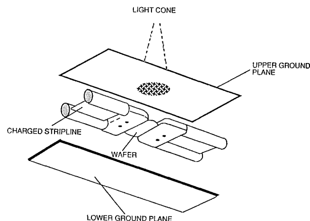
Figure 3. Wafer holder detail.
