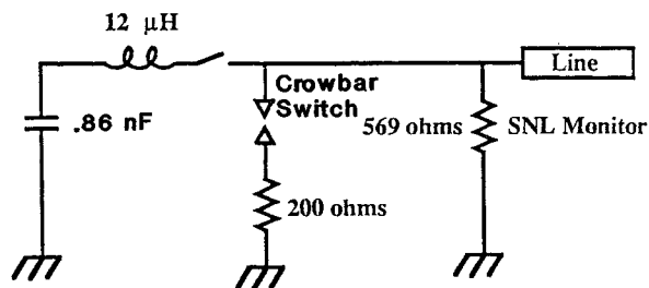
Figure 4. Test circuit.
