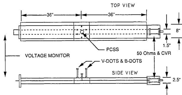
Figure 2. Transmission line test fixture.
