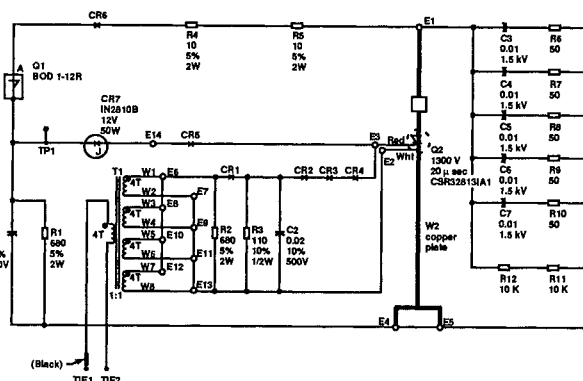
Figure 1. Schematic of circuit card assembly.
