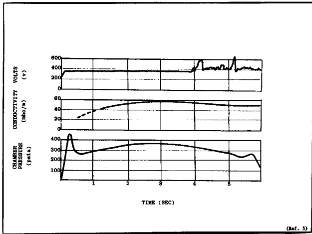
Figure 8. Startup of solid-grain MHD power source.
