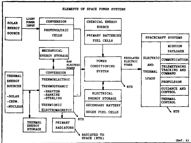
Figure 6. Relationships among various space power systems.
