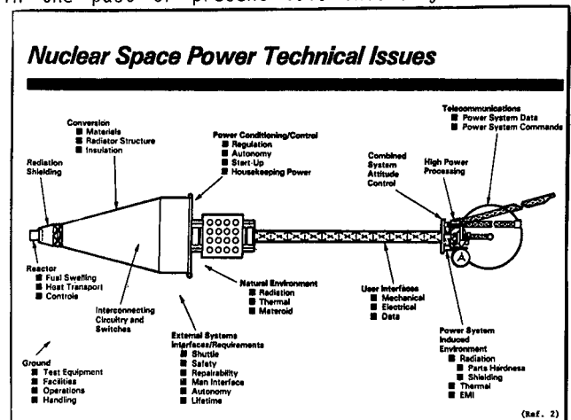
Figure 9. Nuclear space power technical issues.
