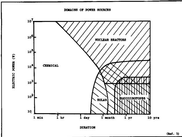
Figure 5. Domains of possible space power sources.
