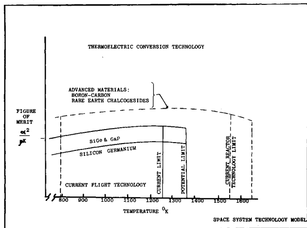
Figure 10. Temporary and efficiency limitations of thermoelectrics.
