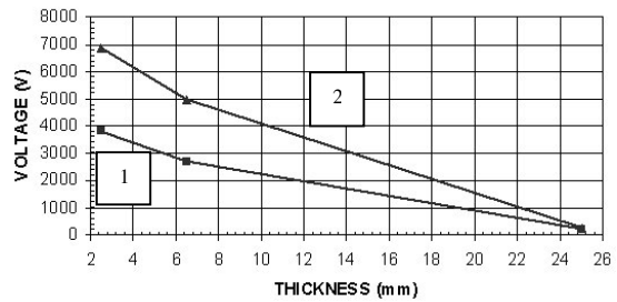
Figure 11. Explosive operation of the EDFEG. The output voltage vs. the thickness of the specimen for 40 \Omega (curve 1) and 400 \Omega (curve 2) loads.
