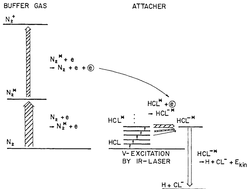
Fig. 7 Energy Level Diagram with Transition Mechanisms for a Gas Mixture with Optically Controlled Attachments
