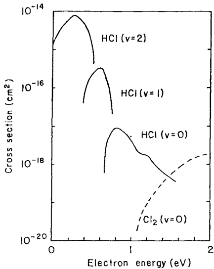
Fig. 6 Dissociative Attachment Cross Sections for Vibrationally Excited HCL Molecules 8
