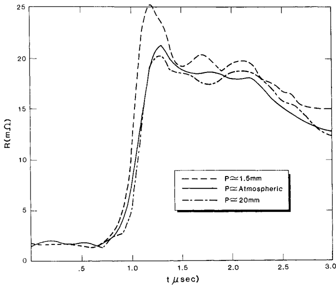
Figure 6. Resistance increase achieved in small scale experiments where the initial air pressure in the switch cavity was varied as indicated.
