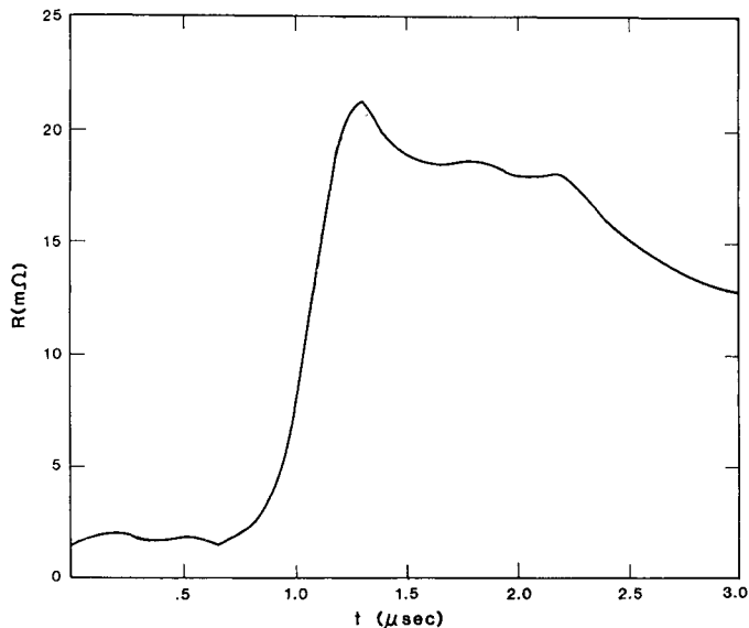
Figure 3. Resistance increase achieved in a typical small scale switch test.
