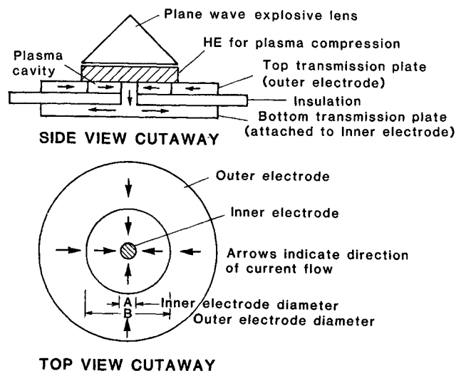
Figure 2. Cutaway sketches showing the side and top views of the new test geometry. Arrows indicate direction of current flow in both views. Dimension A is the diameter of the inner electrode and B is the diameter of the outer electrode.
