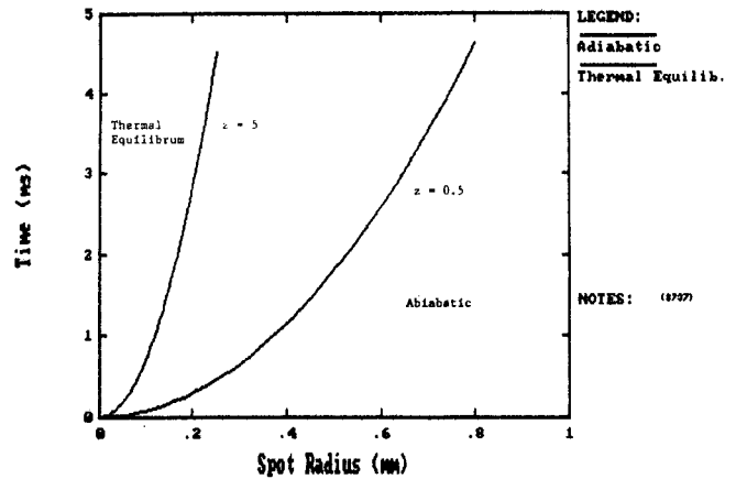
Fig. 1. The contact spot is adiabatic for large spot radius or short times.
