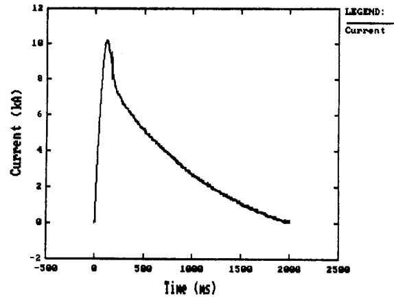
Fig. 4. The current pulse is typically a few milliseconds long.
