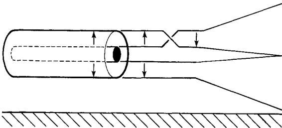
Figure 2. The present PBFA-II configuration has a crossover section that acts like an abrupt impedance transformation. Furthermore, as the gaps between the parallel plates increase energy flows to the exterior of the main lines.
