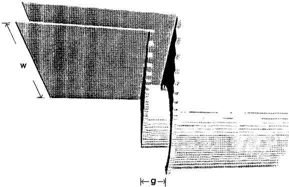
Figure 1. Geometry of the coax-to-parallel-plate transition.
