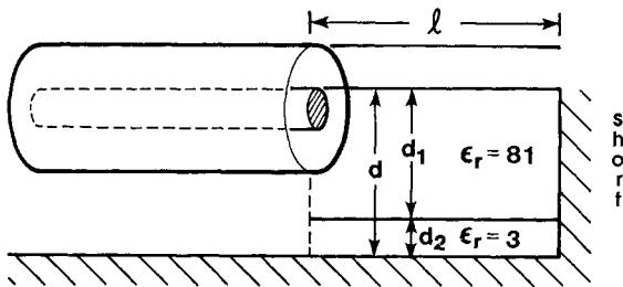
Figure 4. A layer of plastic raises the external impedance in the parallel-plate region. The amount of plastic is chosen to maximize this impedance while insuring transit time isolation between the short and the junction for the duration of the pulse. The two-way transit distance ( 2l ) is 6 m and the pulse duration is 100 ns for PBFA II. This corresponds to 1 m and 16.7 ns respectively for the scale model.
