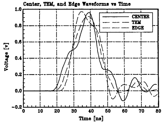
Figure 9. Scale model computer simulations for a 2.54 cm gap (Fig. 1) and a 2.54 cm layer of plastic on the floor.
