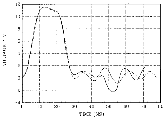
Figure 8. (a) The inlet voltage
