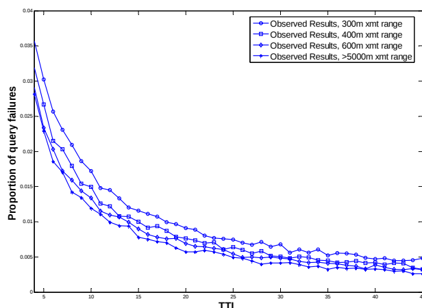
Figure 5: Proportion of query failures, varying node transmission range
