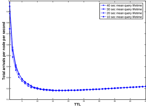
Figure 6: Total arrival rates, varying mean query lifetime
