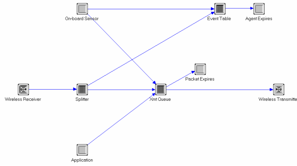
Figure 1: Wireless sensor node model in OPNET
