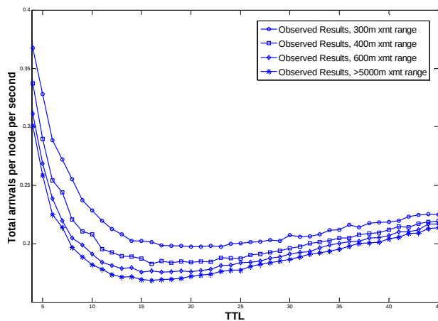
Figure 4: Mean total arrival rates, varying node transmission range
