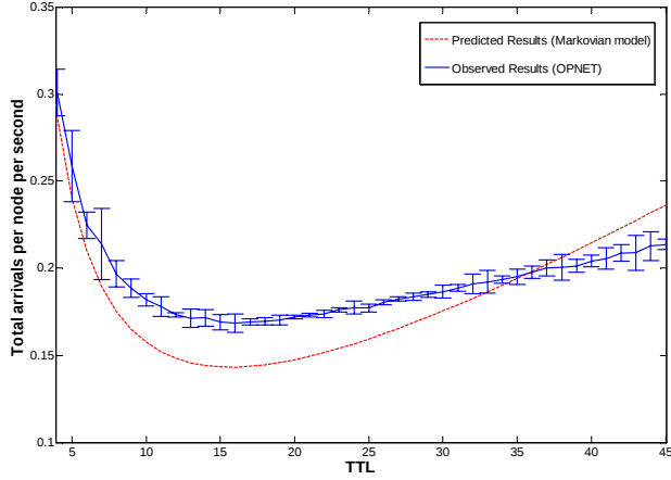
Figure 2: Total arrival rates, infinite transmission range
