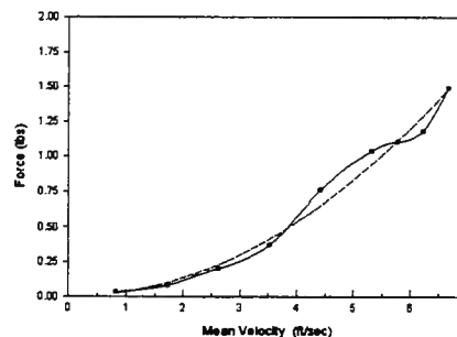
Figure 8 : Side Force versus Mean Velocity
