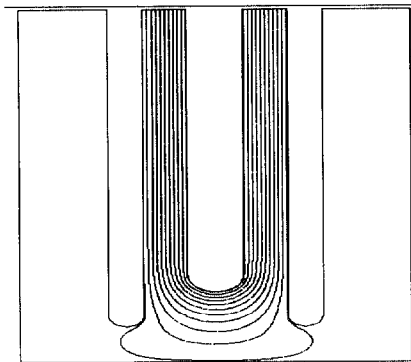
Figure 7. Tri-plate edges have been configured to give reduced E fields on positive plate edges.
