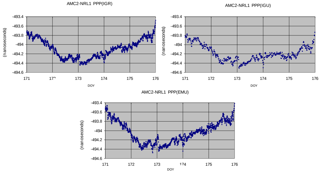
Figure 6. NRCAN PPP 5-day solutions using EMU, IGU, and IGR products differenced between stations.
