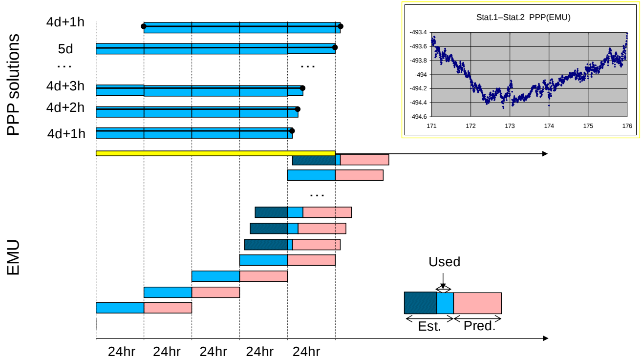
Figure 4. Details of the automated NRCan PPP process using NRCan EMU products with n=4 .
