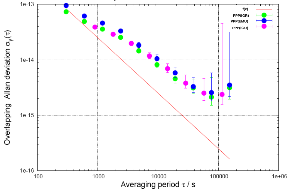
Figure 9. Frequency stability in terms of Allan deviation for the AMC2-NRL1 baseline, for the 2010 DOY 171-175 period.
