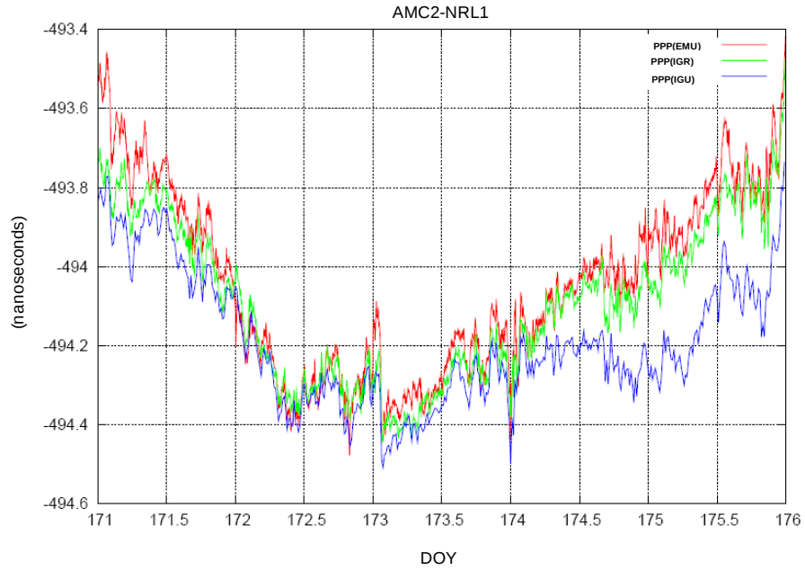
Figure 7. Phase offset for the AMC2-NRL1 baseline, for the 2010 DOY 171-175 period.
