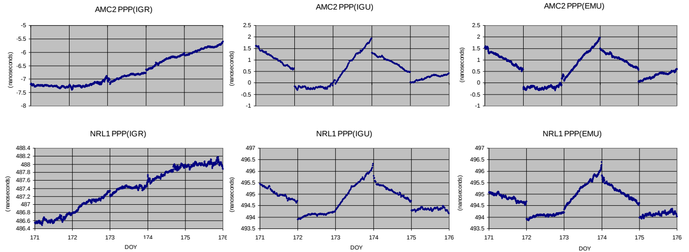
Figure 5. NRCan PPP 5 day solutions using IGR, IGU, and EMU products.
