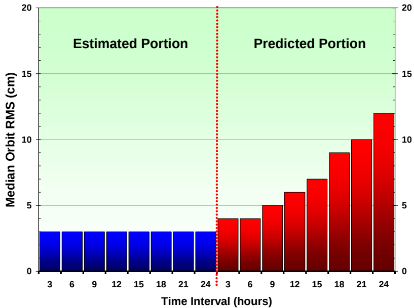
Figure 3. Quality of the NRCAN EMU orbit products, in terms of median orbit RMS with respect to IGS Rapid.
