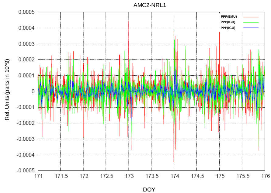
Figure 8. Frequency offset for the AMC2-NRL1 baseline, for the 2010 DOY 171-175 period.
