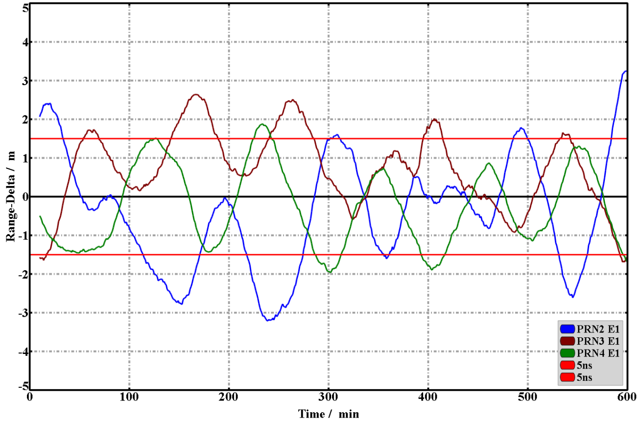
Figure 5. Three of the pseudolites' timing receivers running "uncoordinated" within 10 hrs.
