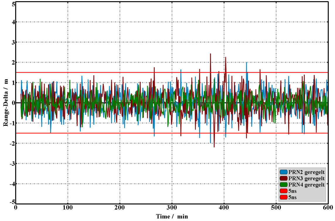
Figure 6. The same receivers with a 10 min control time constant, including noise.
