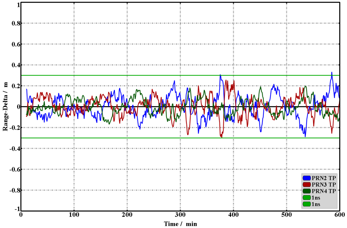
Figure 7. The same receivers with a 10 min control time constant (results low pass filtered).
