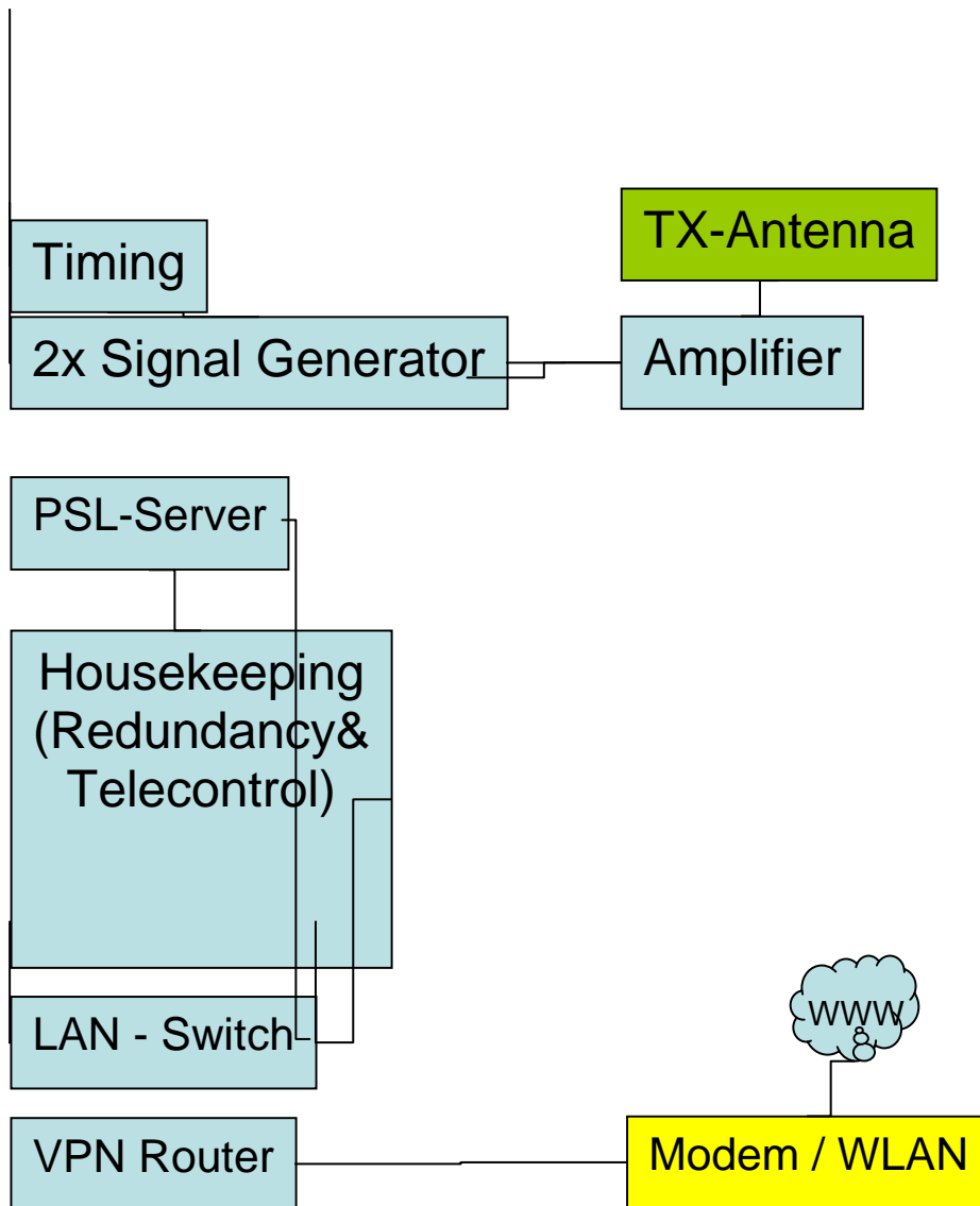
Figure 4. Block diagram of a pseudolite.
