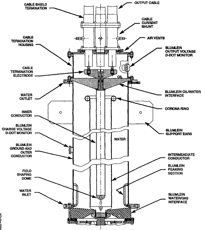
Figure 7. Blumlein cross section.
