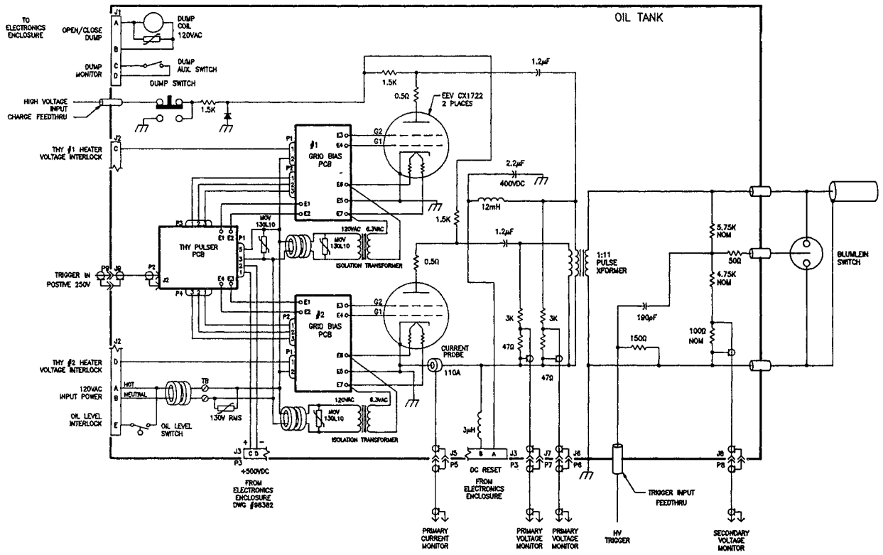
A SINGLE BLUMLEIN CHARGING UNIT SHOWN (TYPICAL OF 4 UNITS)
