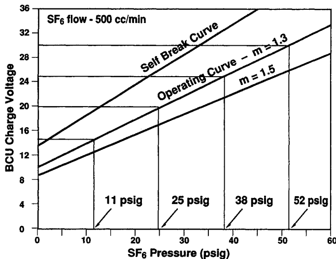
Figure 10. Blumlein switch SF 6 operating pressure (m = 1.3) curve.
