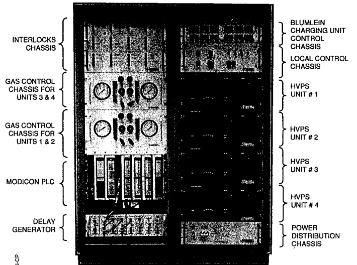
Figure 2. ICPPS Control Console.
