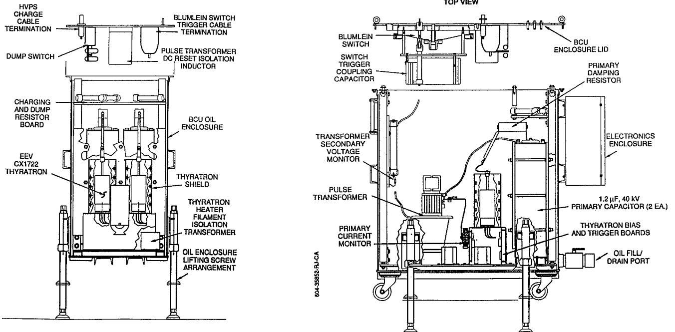
Figure 3. Blumlein Charging Unit showing component layout.
