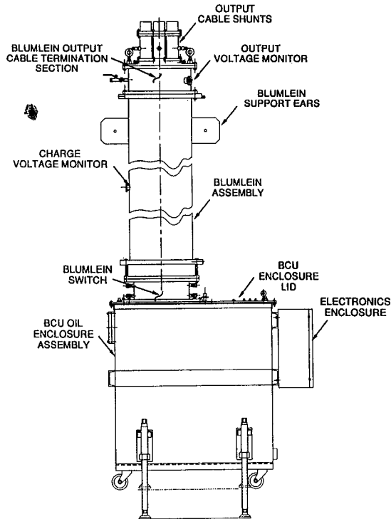
Figure 1. A single Blumlein/BCU.
