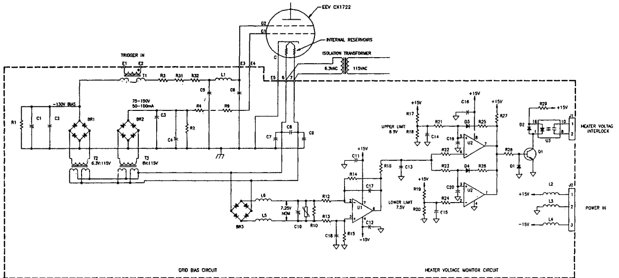
Figure 5. Thyatron biasing and trigger circuit schematic.
