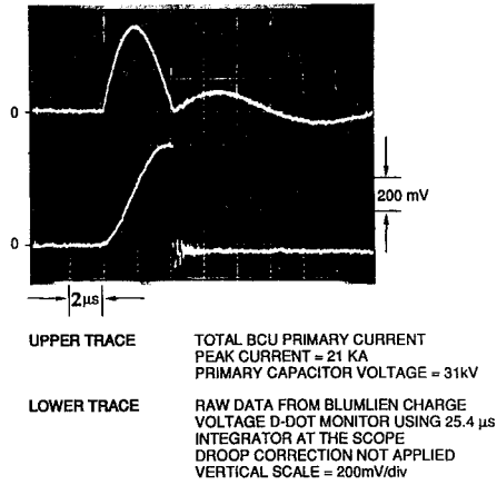
Figure 6. Primary current and charging voltage.
