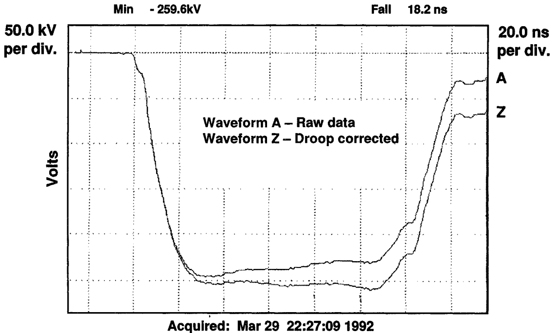
Figure 8. Blumlein output pulse into matched load.
