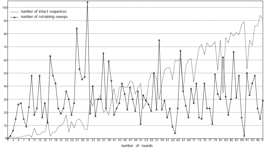
Fig. 3. The number of intact sequences and the number of retraining sweeps with respect to training rounds during training with the Table 1 database.
