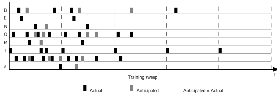
Fig. 2. Training and generation of the sequence \langle TO - BE - OR - NOT - TO - BE \rangle . The activity traces of the input terminals are shown, where a black box represents an actual terminal activity, a gray box represents an anticipated activity that does not match the actual input, and a white box represents a match between an anticipated and an actual input activity. The training phase takes 5 training sweeps. The generation process is initiated by presenting the first component of the sequence, T . The parameter values used are: \alpha = 0.2 , \delta = 0.1 , and C = 3.0 .
