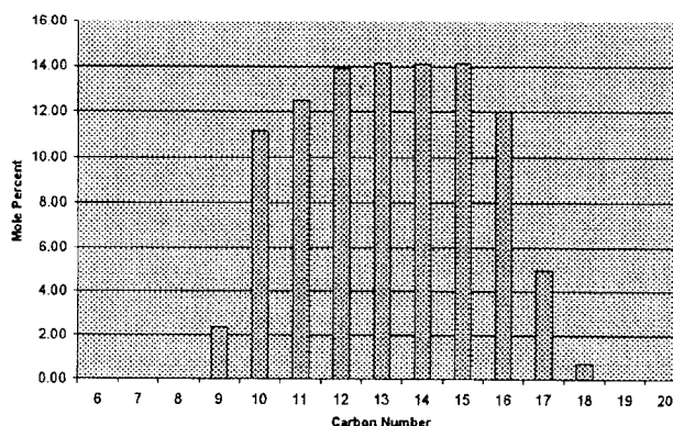
Figure 4. Paraffinic Hydrocarbon Distribution by Carbon Number for Syntroleum S-5 Synthetic Jet Fuel
