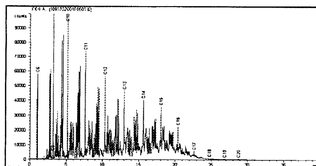
Figure 3. HP 5890 Analytical GC Trace of Syntroleum S-5 Synthetic Jet Fuel with Normal Paraffinic Hydrocarbons Labeled
