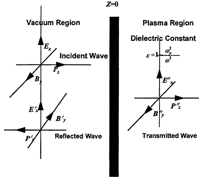
Figure 3. Wave Reflection at Vacuum/Plasma Interface
