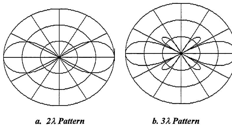
Figure 8. Computed Radiation Patterns for Plasma Line Antenna
