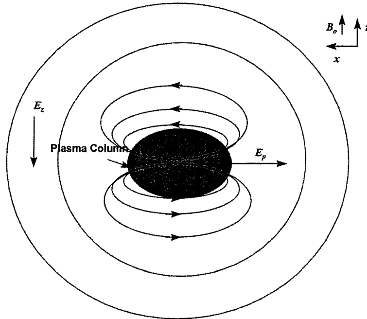
Figure 1. Radiation Pattern of Plasma Column
