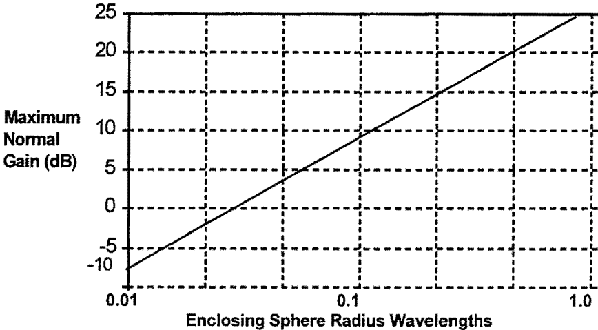
Figure 2. Antenna Supergain Curve
