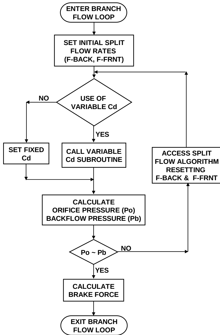
Figure 31. Detail Flowchart of Recoil Pressure/Force Calculations
