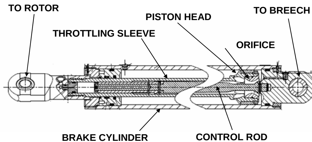
Figure 19. Assembly View of XM360 Recoil Brake
