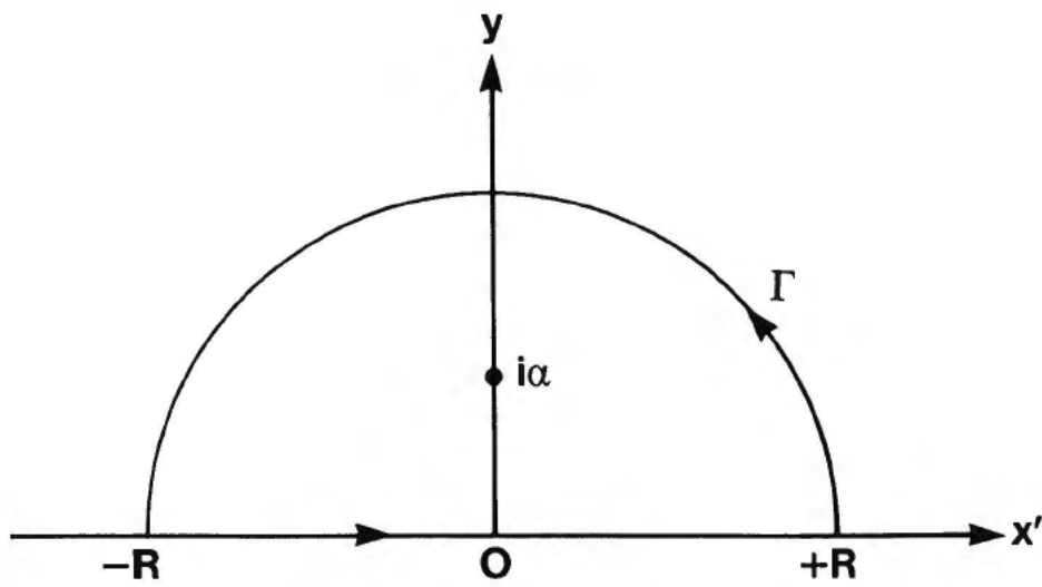
Figure 3 Contour of Integration (No poles on the Real Axis) in the Complex z -Plane
