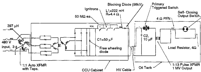
Figure 2. Equivalent circuit of command charging unit and pulser
