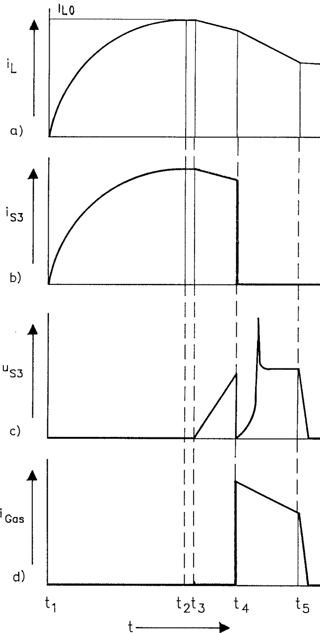
Fig. 2: Current and voltage waveforms in the inductive storage circuit
