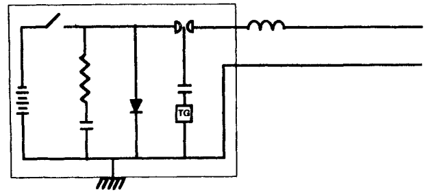
Figure 9 SPEAR II High Current Schematic
